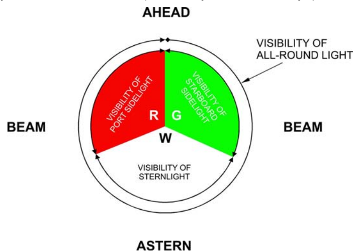
Figure 7 Arc of Visibility
