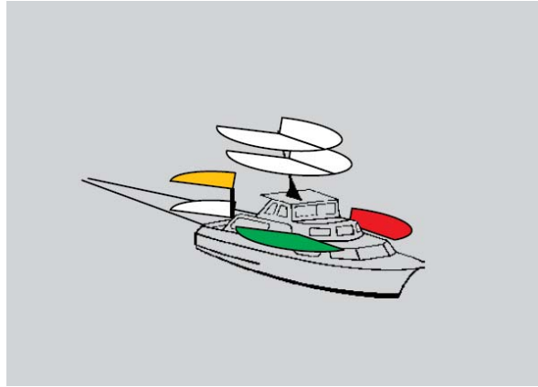
Figure 10 Towing Vessel
