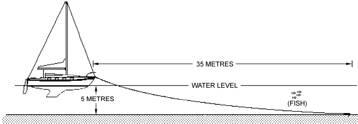
Figure 4 Anchor Scope
